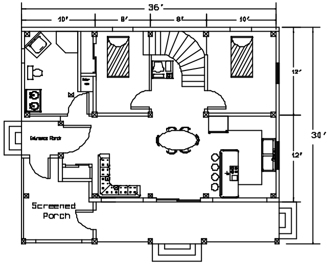
Main Level 30x36 collage floor plan
