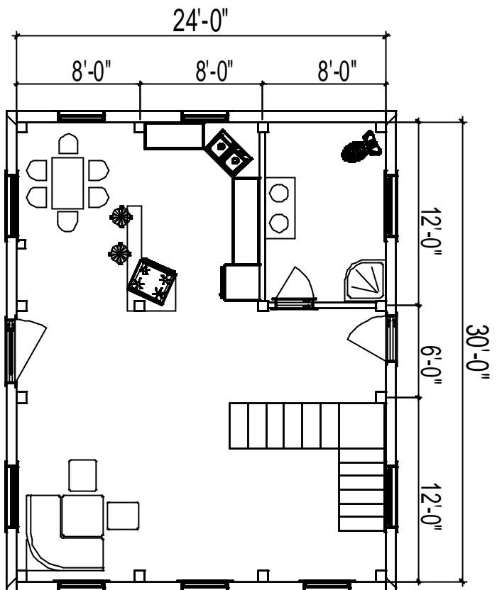
proposed floor plan (main floor) for the 24X30 chalet
